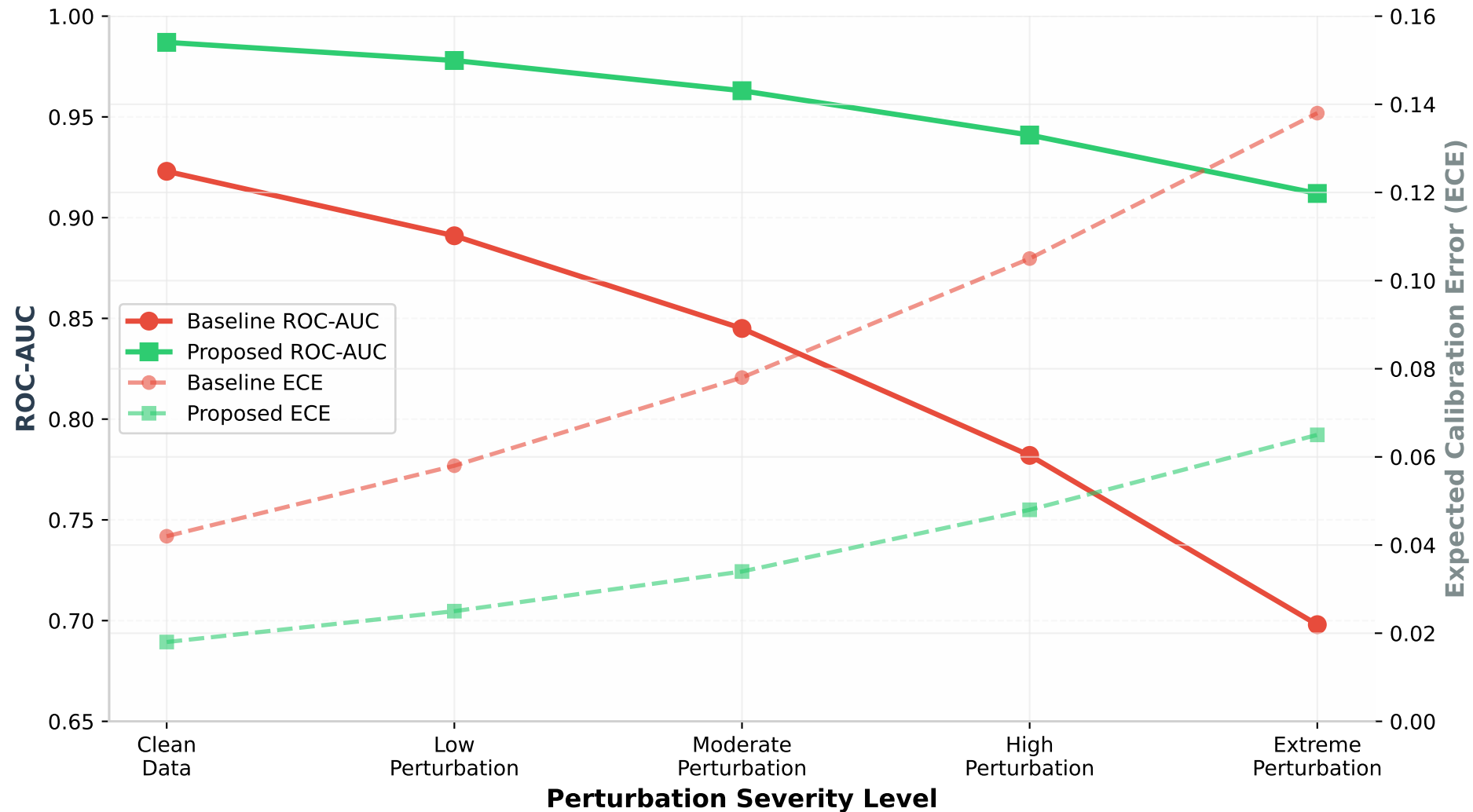
Robustness Degradation Under Increasing Data Perturbations
